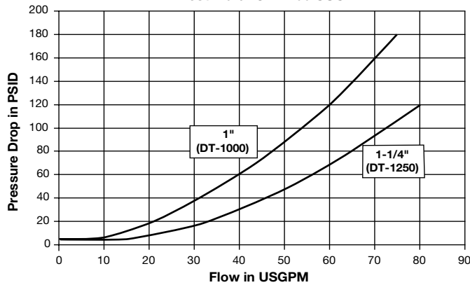
DT Series (1" & 1-1/4") Test Fluid: Oil - 200 SUS
